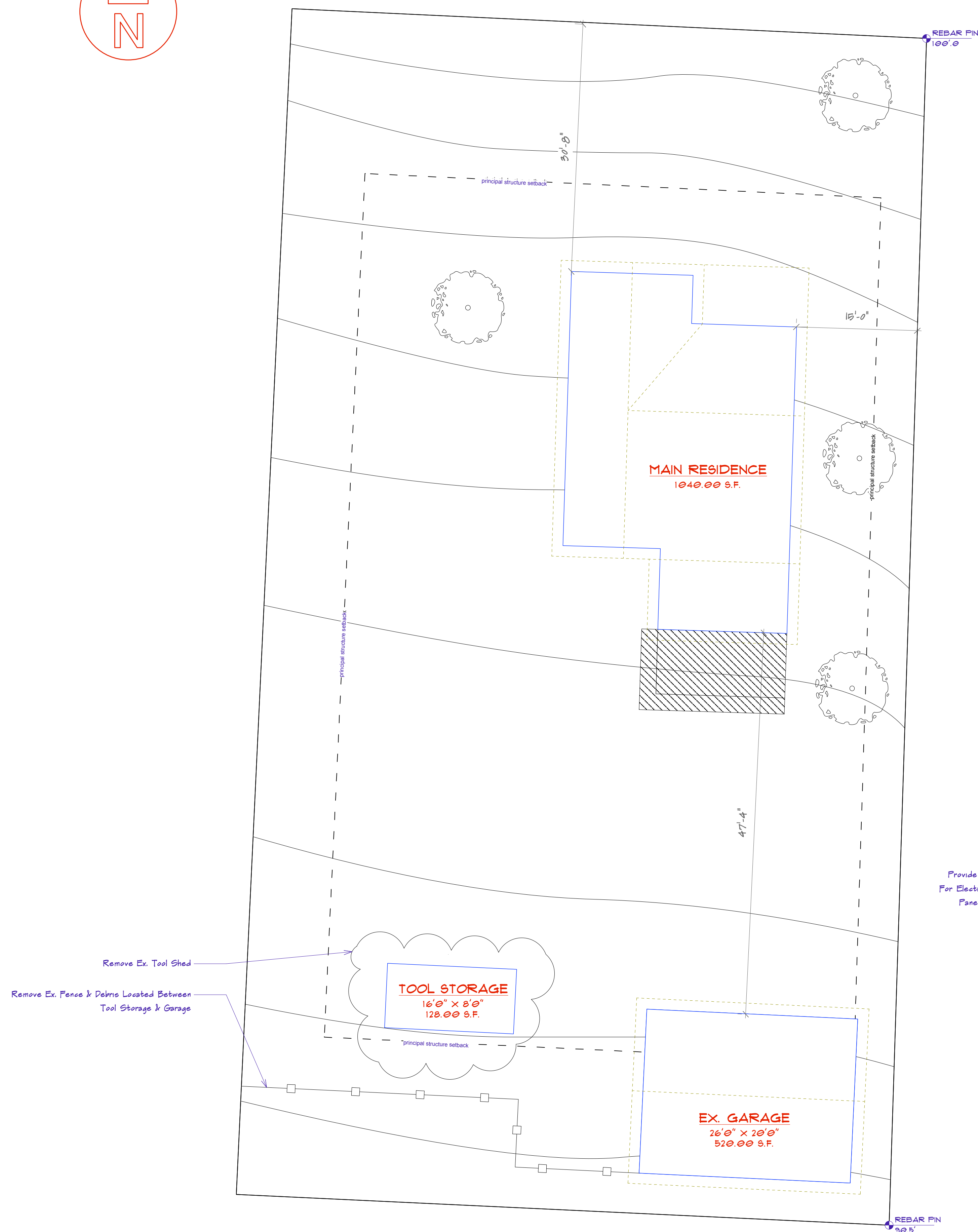
1 EX. PLOT PLAN SCALE: 1/8" = 1'-0"
