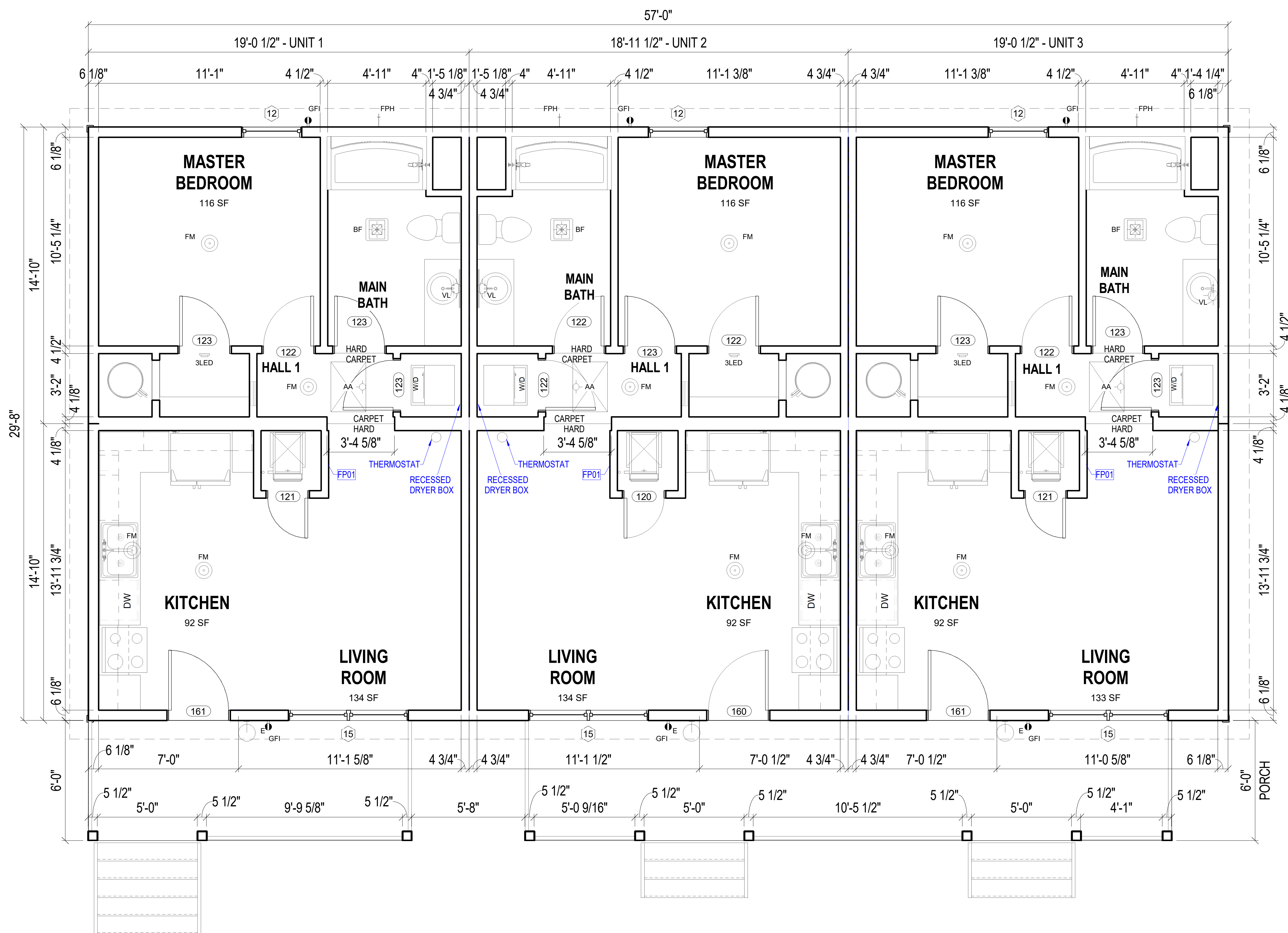
FLOOR PLAN
